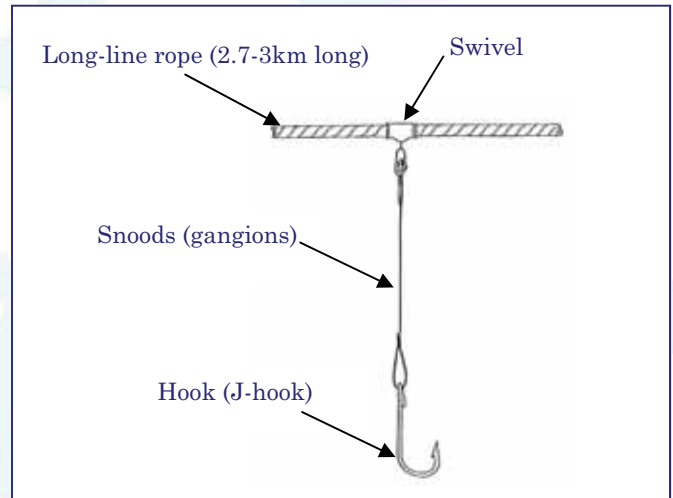
Fig. 3. Long-line configuration. The hooks (size 7 or 9) were baited with 20-40g of Sardina philchardus .
